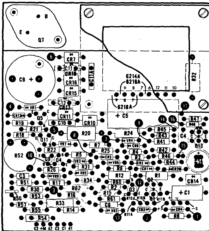
Figure A-2. Model 6216B, Component Location Diagram
