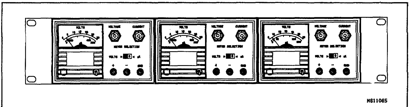
Figure 2-2. Rack Kit with Three Bench Supplies
