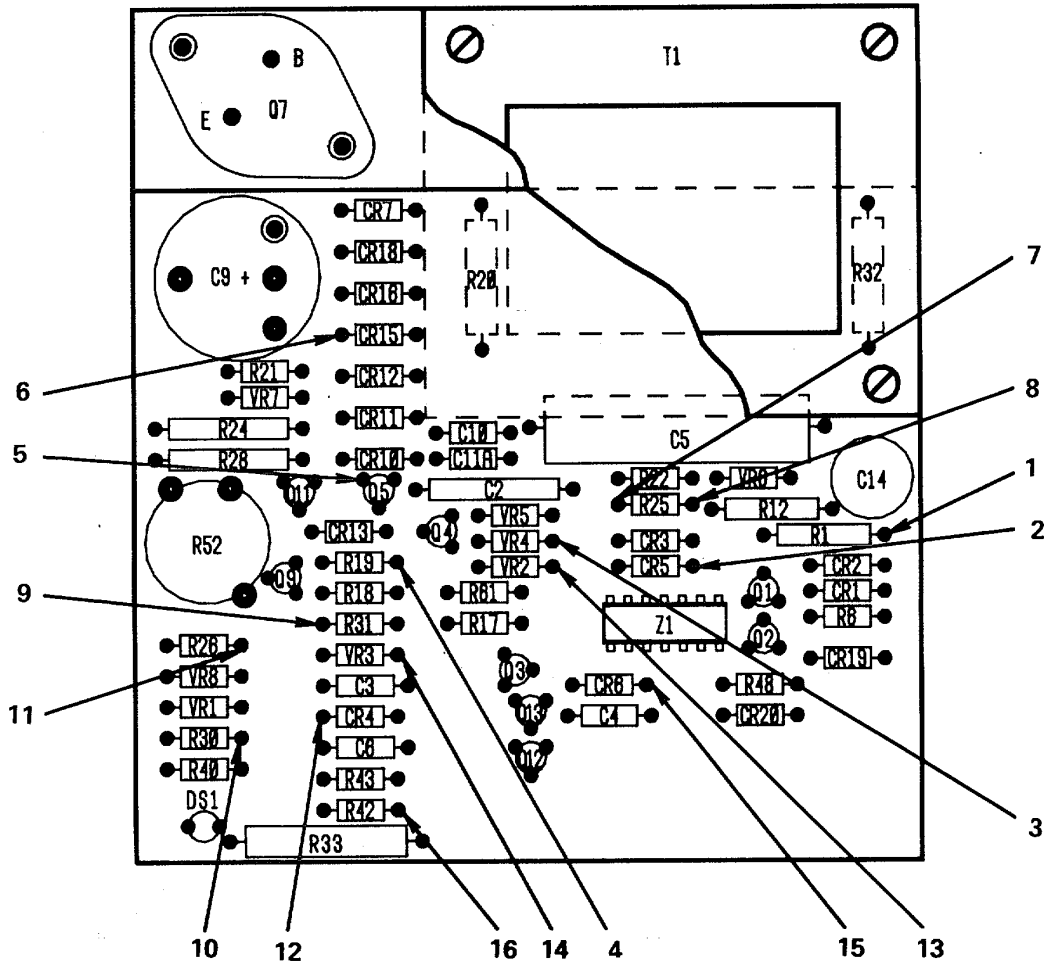
Figure A-1. Model 6216B, Components Location Diagram
