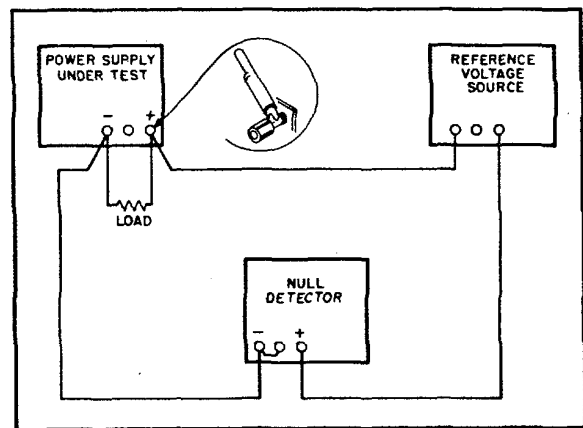
Figure 5-1. Differential Voltmeter Substitute Test Setup
