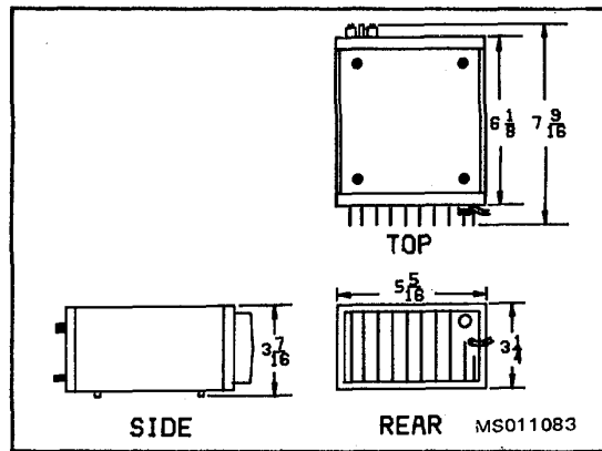
Figure 2-1. Outline Diagram
