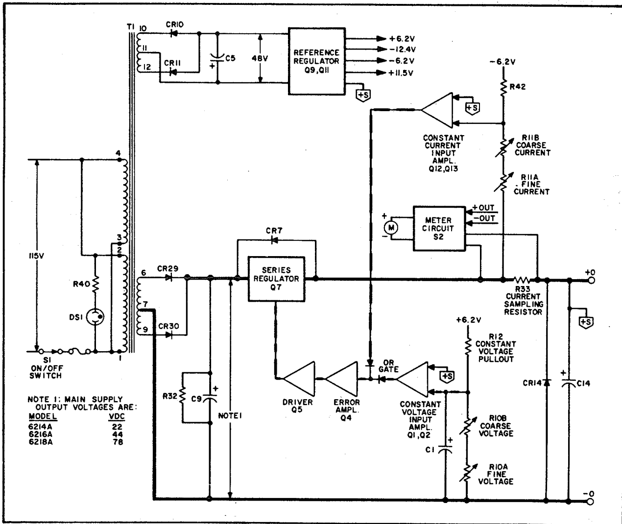
Figure 4-1. Block Diagram
