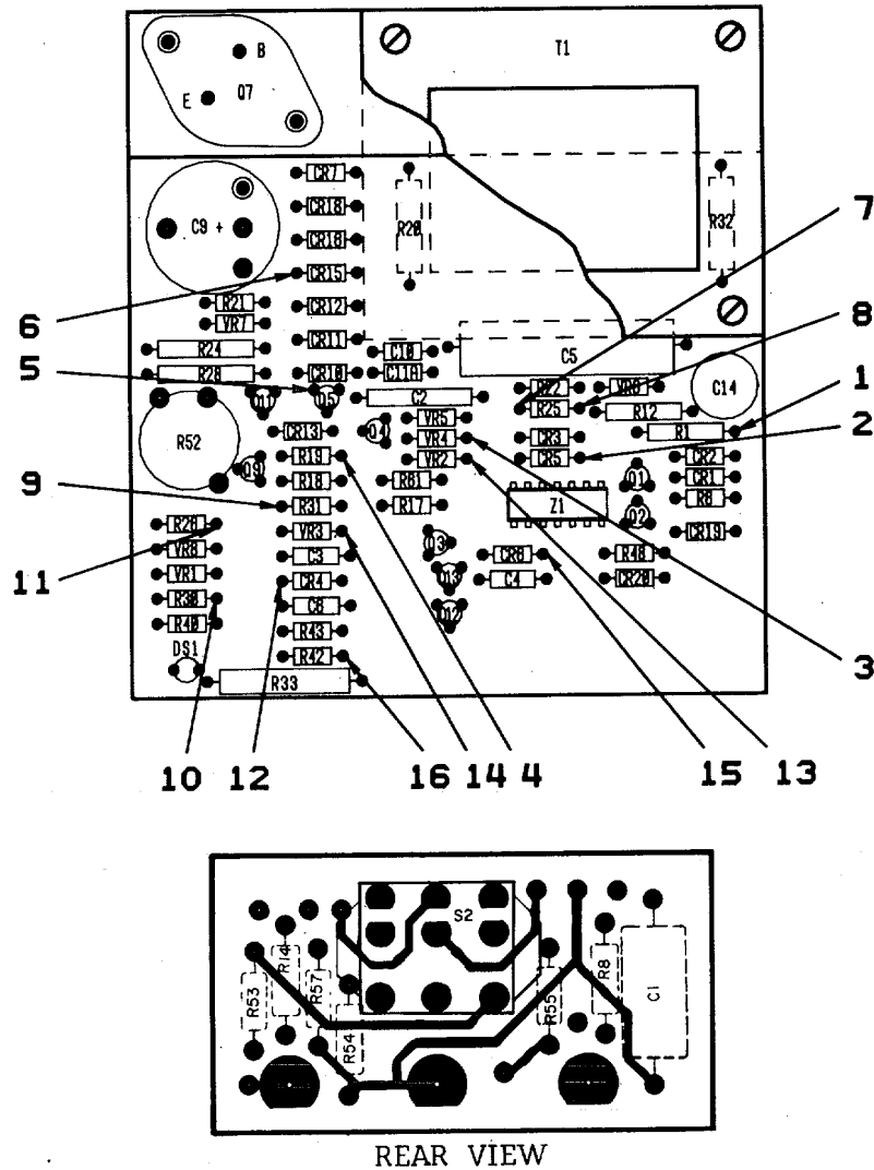
Figure 7-1. Model 6216B Component Location Diagram
