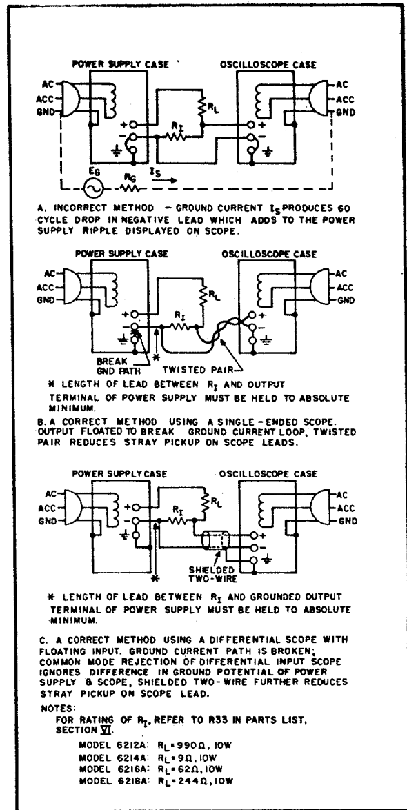
Figure 5-11. CC Ripple and Noise Test Setup
