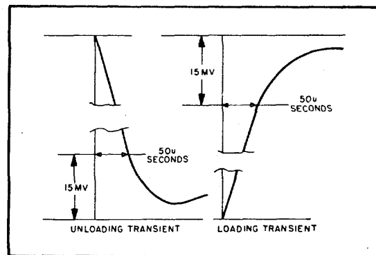
Figure 5-8. Transient Recovery Time, Waveforms
