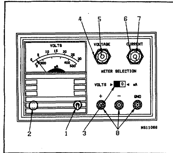
Figure 3-1. Front Panel Controls and Indicators
