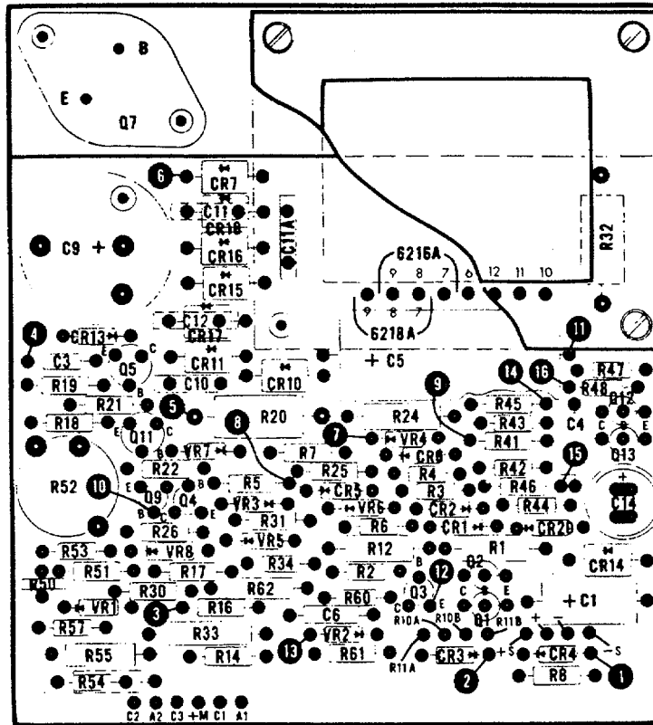
Figure A-3. Model 6216B, Component Location Diagram
